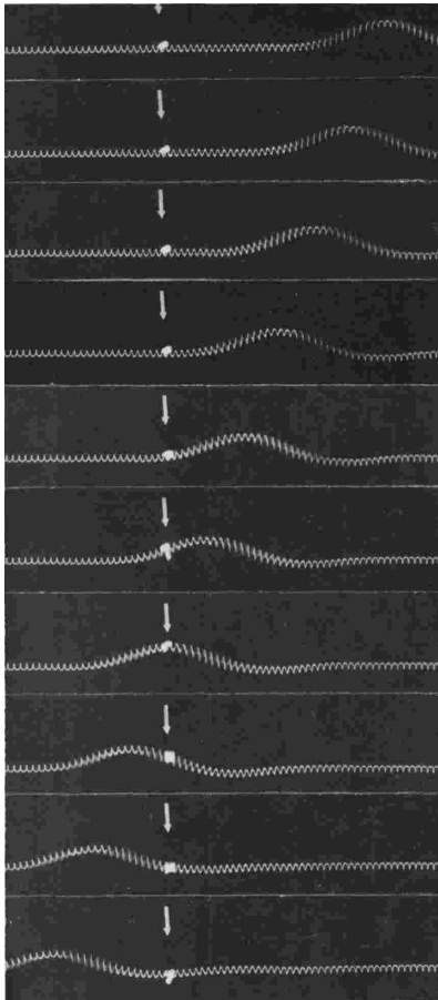
d / As the wave pulse goes by, the ribbon tied to the spring is not carried along. The motion of the wave pattern is to the right, but the medium (spring) is moving from side to side, not to the right. ( PSSC Physics )
